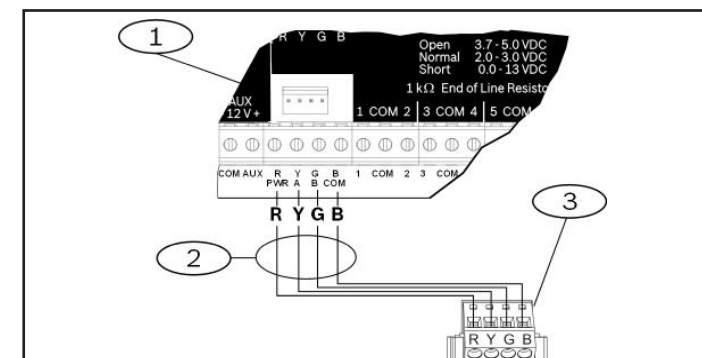
Figure 3.1: Wiring the keypad to the SDI2 bus connection (B5512 shown)
