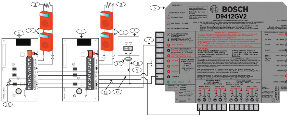
Figure 5.3: Wiring interconnected modules to a G Series panel with power supplied by an external power supply
