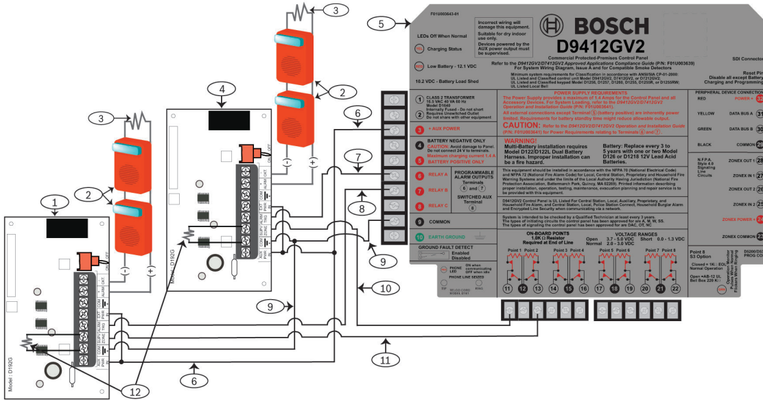
Figure 5.4: Wiring separate module loops to a G Series panel with power supplied by an external power supply
