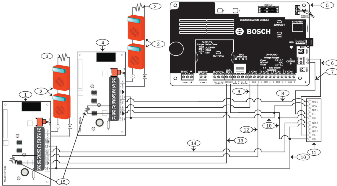
Figure 5.6: Wiring separate module loops to a B Series control panel supplying 12 VDC power
