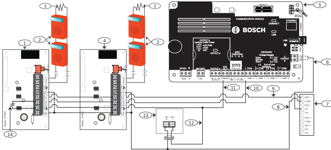
Figure 5.7: Wiring interconnected modules to a B Series panel with power supplied by an external power supply
