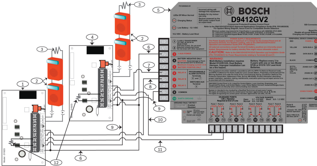
Figure 5.2: Wiring separate module loops to a G Series control panel supplying 12 VDC power
