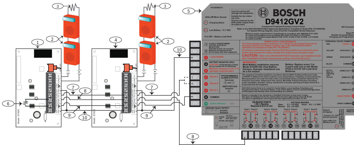
Figure 5.1: Wiring interconnected modules to a G Series panel supplying 12 VDC power
