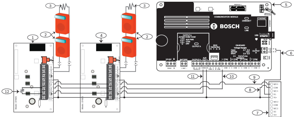
Figure 5.5: Wiring interconnected modules to a B Series panel supplying 12 VDC power
