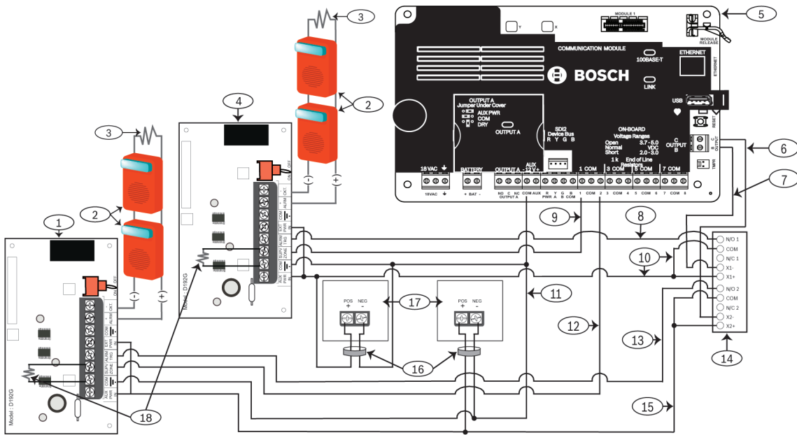
Figure 5.8: Wiring separate module loops to a B Series panel with power supplied by an external power supply
