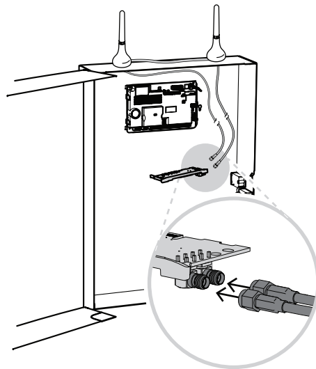
Figure 3.4: B444-A/B444-V cable connection
