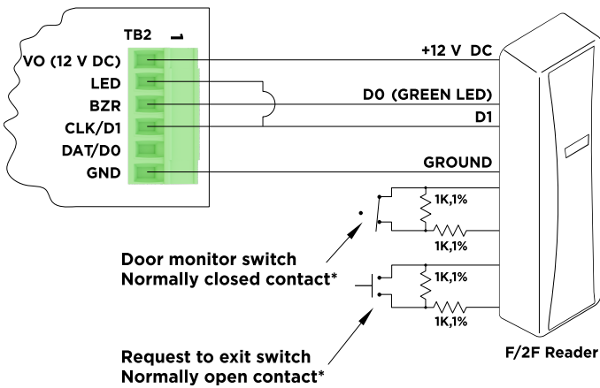
Reader port 1 Typical supervised F/2F reader
