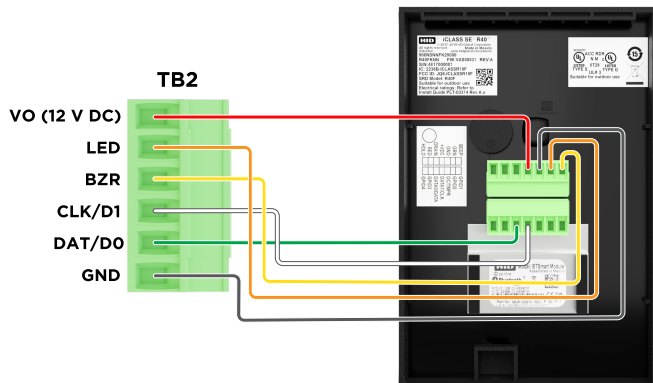
Reader port 1, typical reader 2 (Wiegand or Clock/Data installation)
