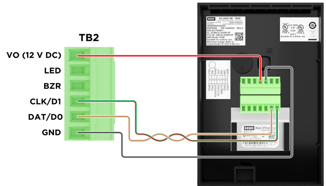
Reader port 1, typical reader 1 (OSDP installation)
