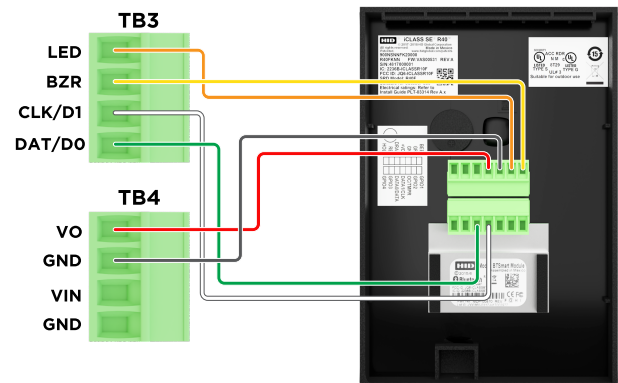
Reader port 2, typical reader 2 (Wiegand or Clock/Data installation)
