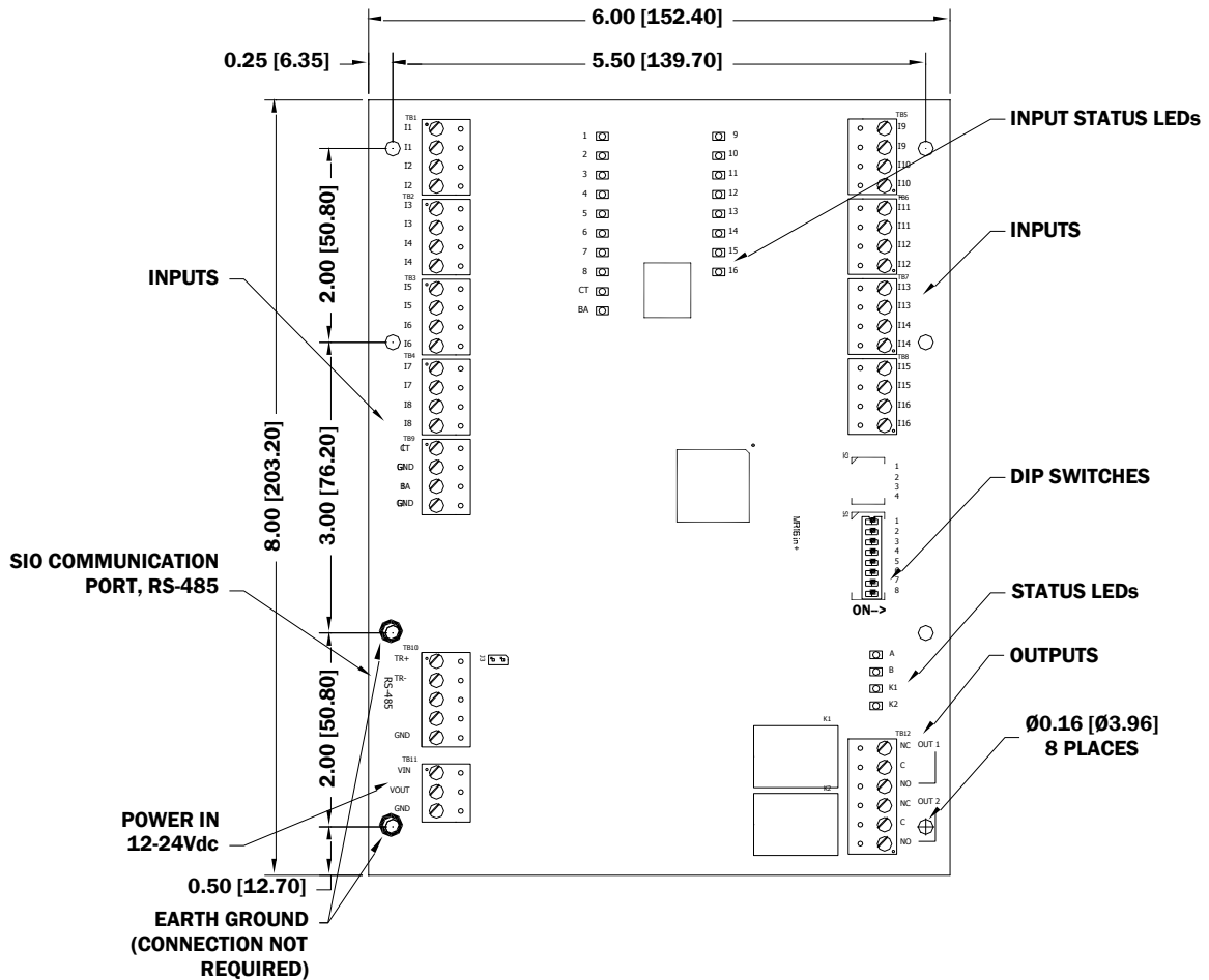
MR16in-S3 Layout
