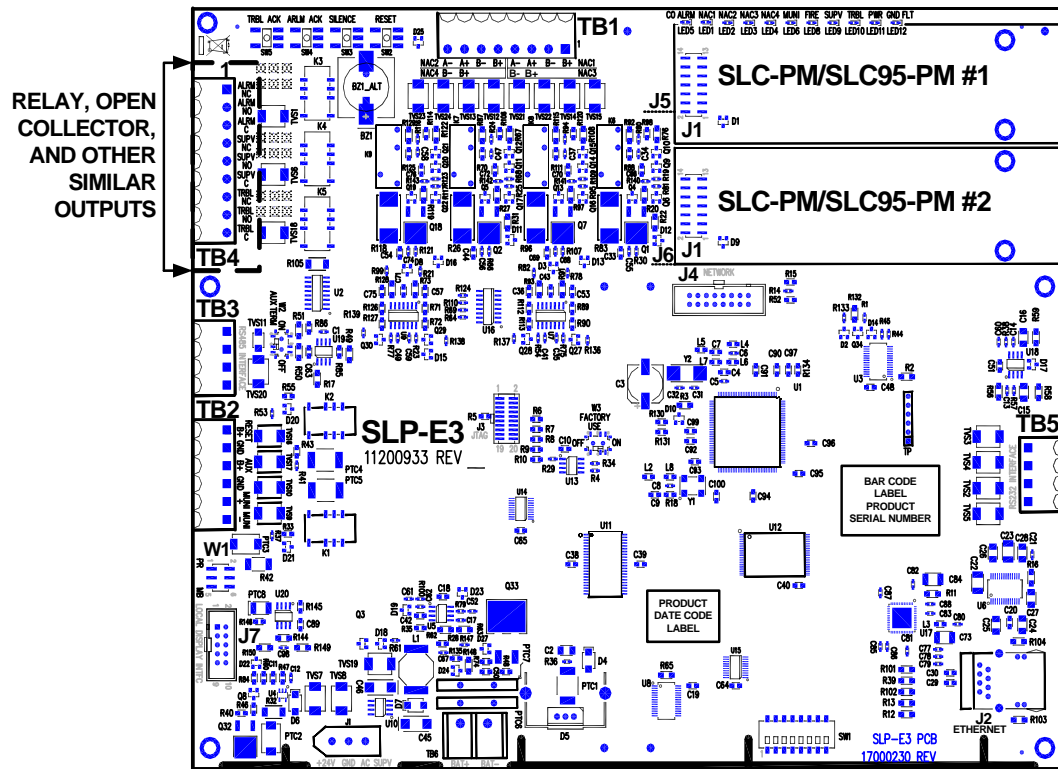
Figure 2.13.1 Relay, Open Collector and Other Outputs
