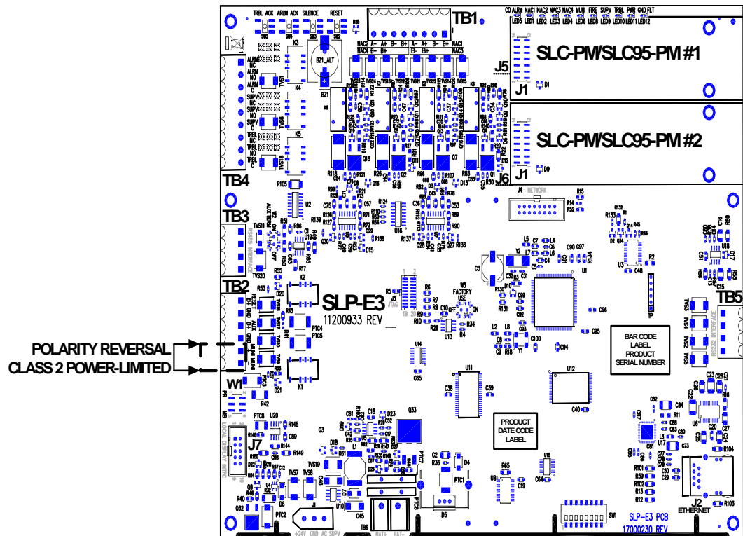
Figure 2.8.1 Reverse Polarity Communication Line Circuit
