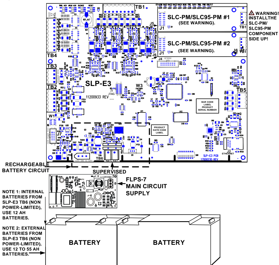
Figure 2.2.2.1 SLP-E3 Rechargeable Battery Installation Wiring Diagram
