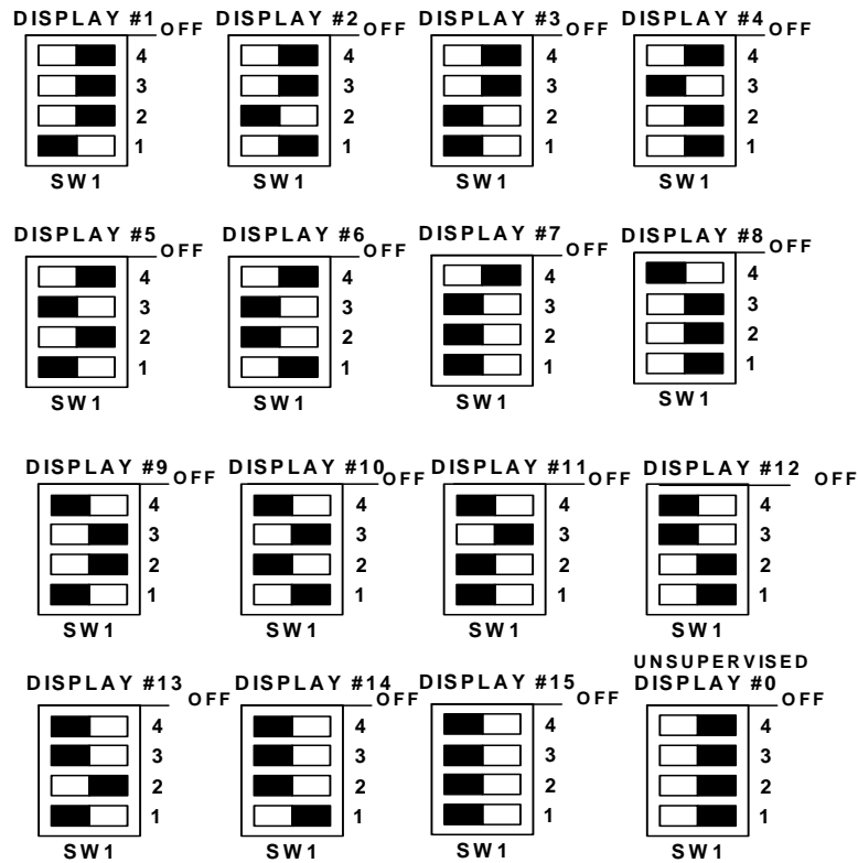
Figure 2.7.11.1 Binary Switches
