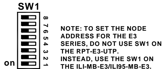
Figure 2.10.5.2 E3 Series, ILI-MB-E3/ILI95-MB-E3/NGA Address Settings
