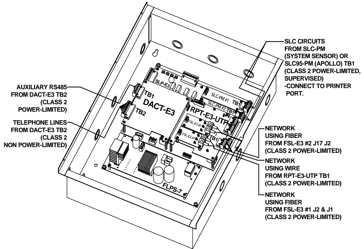
Figure 2.15.1.2 S3 Series, SLP-BB Cabinet, Class 2 Power-Limited and Non-Power-Limited Wiring (Optional Top Level Circuit Board Configuration)
