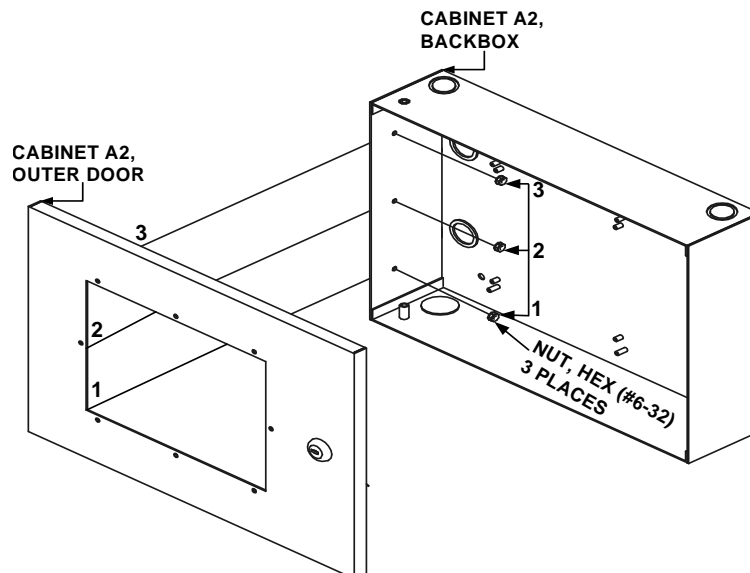
Figure 2.18.1.1.1 E3 Series Cabinet A2, Outer Door to Backbox Installation
