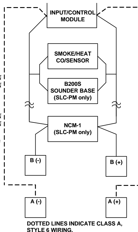
Figure 2.6.1.1 Signaling Line Circuits
