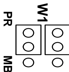
Figure 2.8.1.1 W1 Jumper Block Positions for Polarity Reversal
