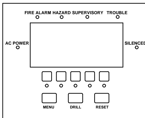
Figure 3.1.4.1 LCD-SLP Switches
