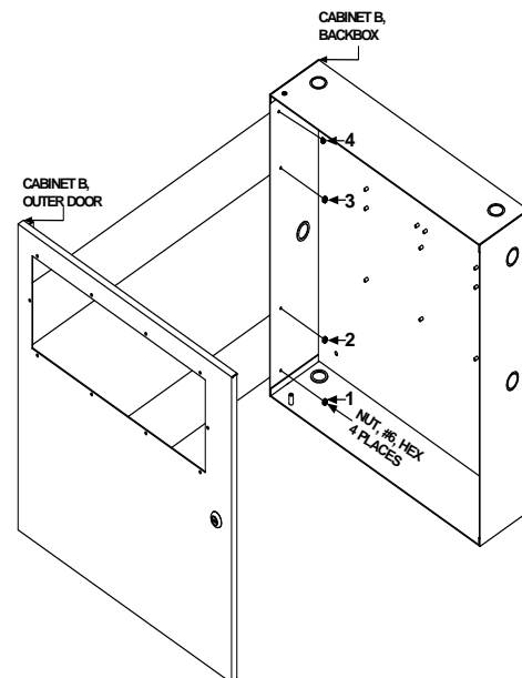
Figure 2.16.1.2 S3 Series Cabinet B, Outer Door to Backbox Installation
