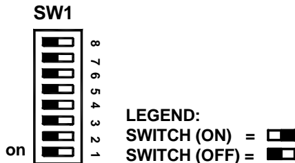
Figure 2.10.5.1 Standalone Address Settings
