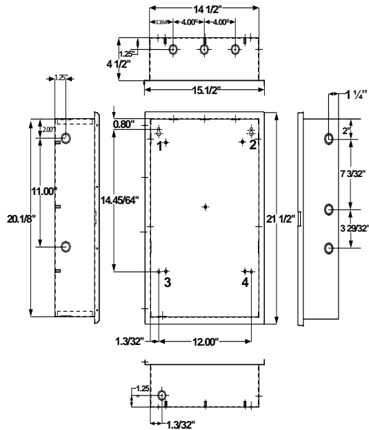
Figure 2.14.1.1 SLP-BB Cabinet Dimensions
