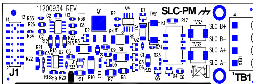
Figure 2.6.2.1 SLC-PM Circuit Board
