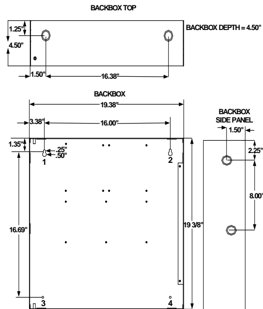
Figure 2.16.1.1 S3 Series, B-Size Cabinet Dimensions
