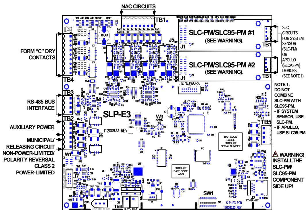
Figure 2.2.1 SLP-E3 Main Circuit Board
