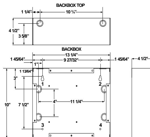
Figure 2.19.1.1 E3BB-FLUSH-LCD Cabinet A2 Dimensions
