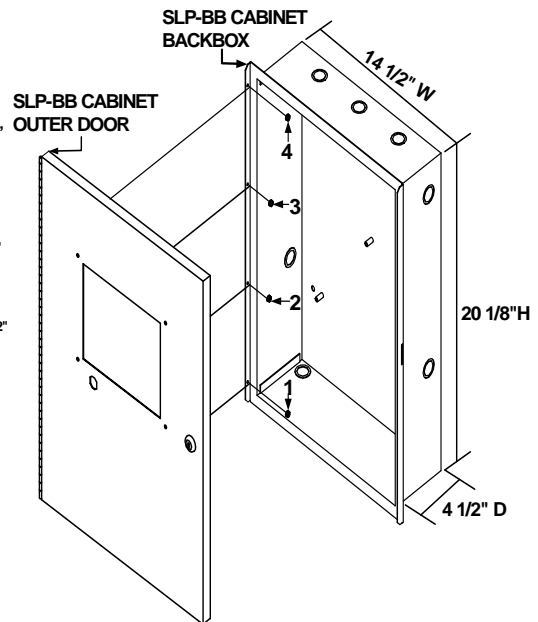
Figure 2.14.1.2 SLP-BB Outer Door to Backbox Assembly
