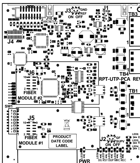
Figure 2.10.3.1 RPT-E3-UTP Circuit Board Diagram
