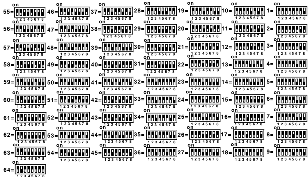
Figure 2.10.5.3 S3 Series Panel Node Address Switch Settings
